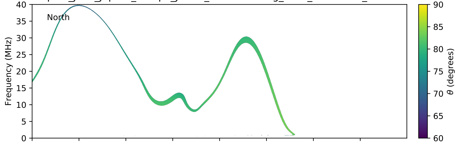
expres_juno_jupiter_europa_jrm09_lossc-wid1deg_3kev_20190202_v01.cdf
