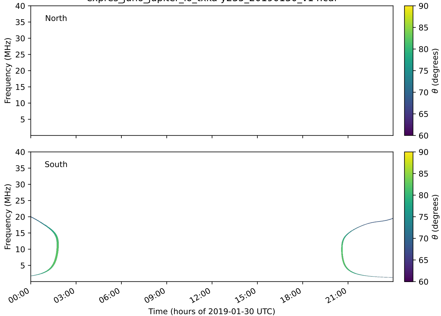
expres_juno_jupiter_io_txka-y235_20190130_v14.cdf
