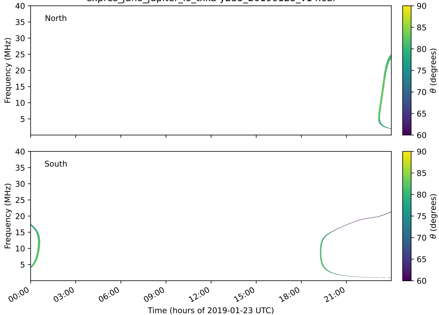
expres_juno_jupiter_io_txka-y235_20190123_v14.cdf
