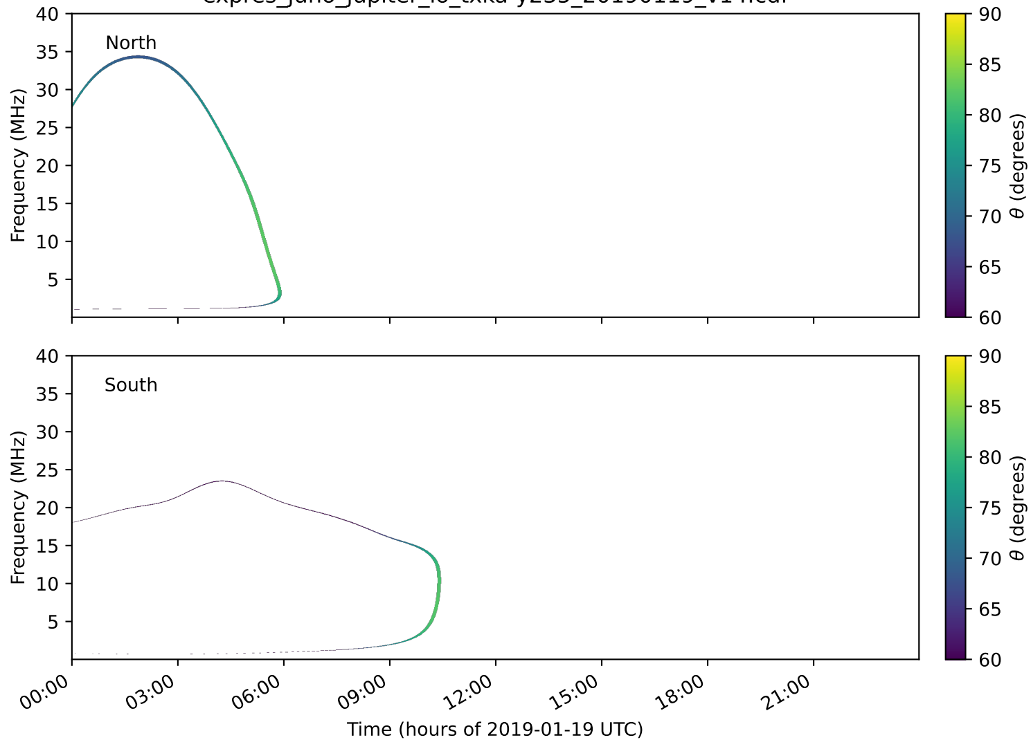
expres_juno_jupiter_io_txka-y235_20190119_v14.cdf
