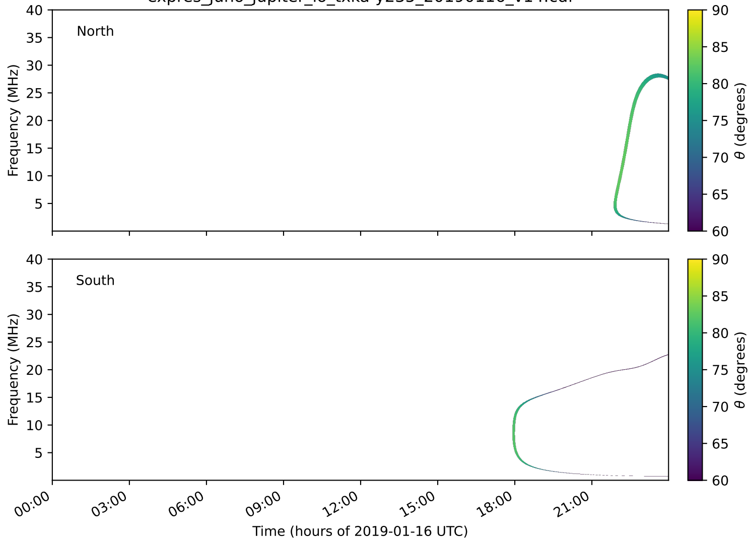
expres_juno_jupiter_io_txka-y235_20190116_v14.cdf
