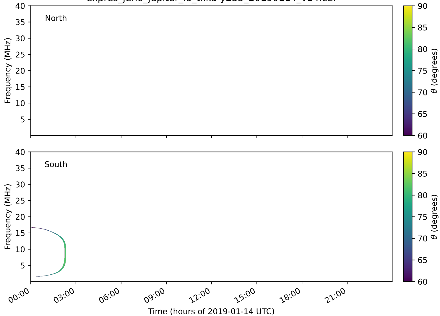
expres_juno_jupiter_io_txka-y235_20190114_v14.cdf
