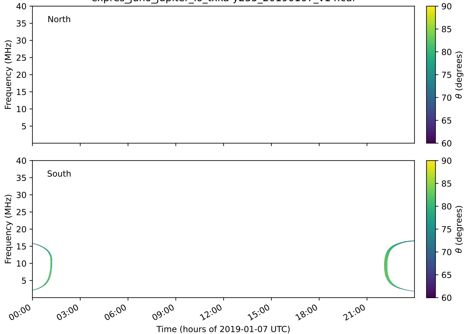
expres_juno_jupiter_io_txka-y235_20190107_v14.cdf
