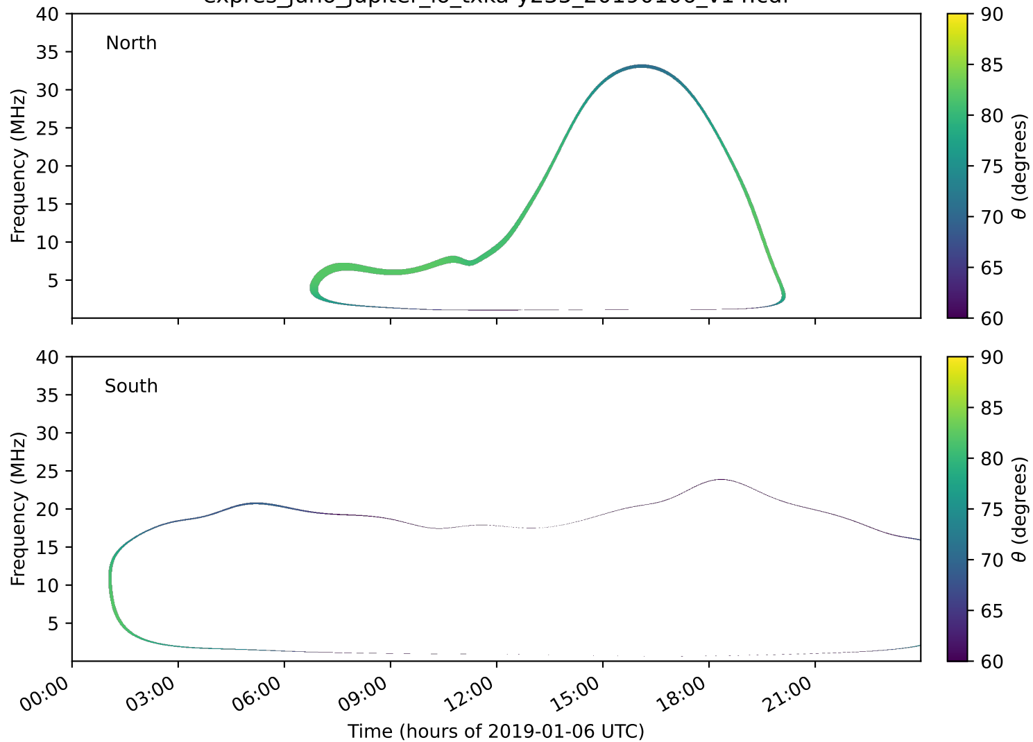
expres_juno_jupiter_io_txka-y235_20190106_v14.cdf
