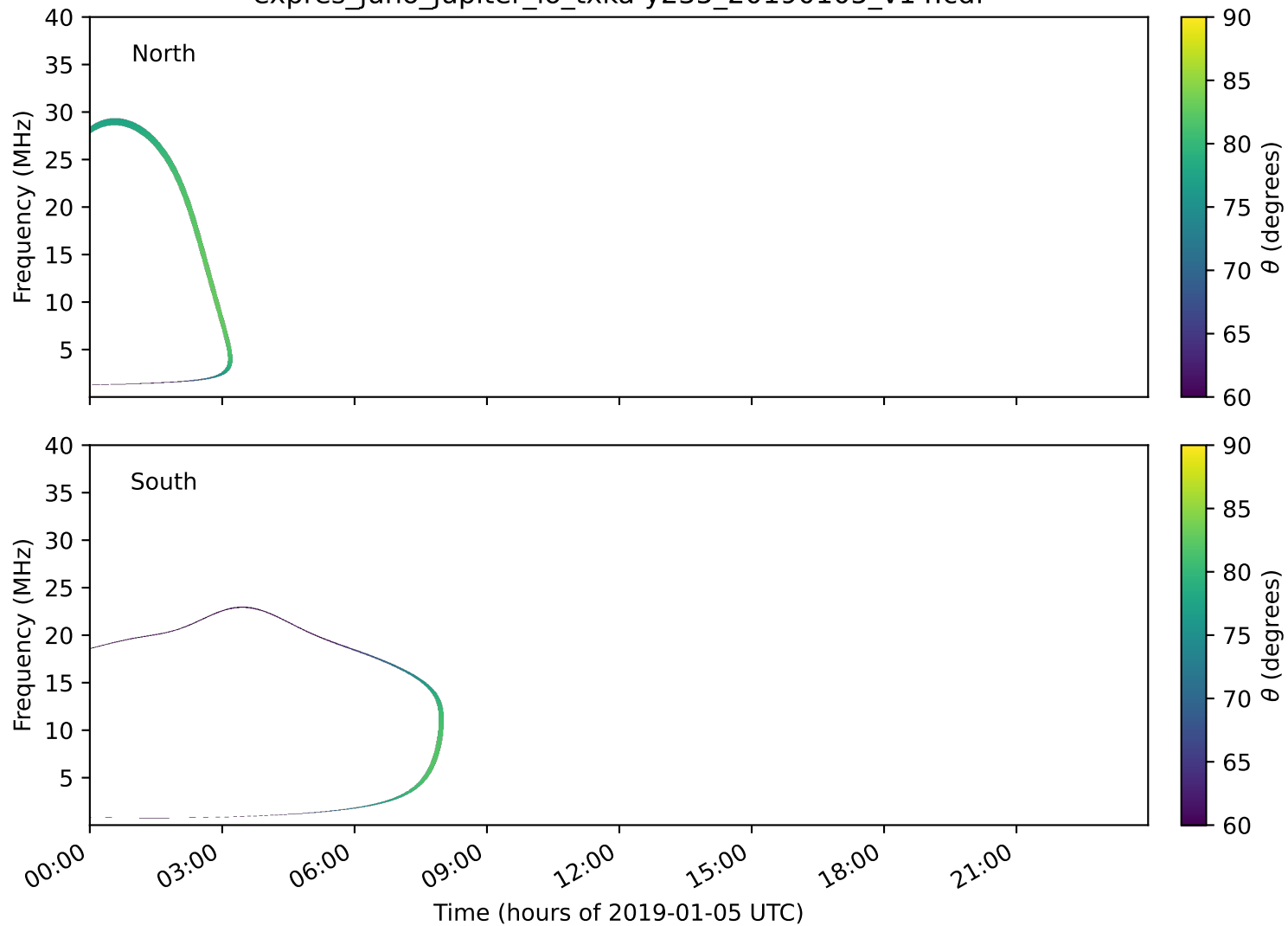
expres_juno_jupiter_io_txka-y235_20190105_v14.cdf
