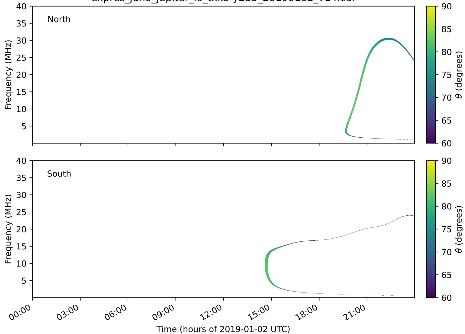
expres_juno_jupiter_io_txka-y235_20190102_v14.cdf
