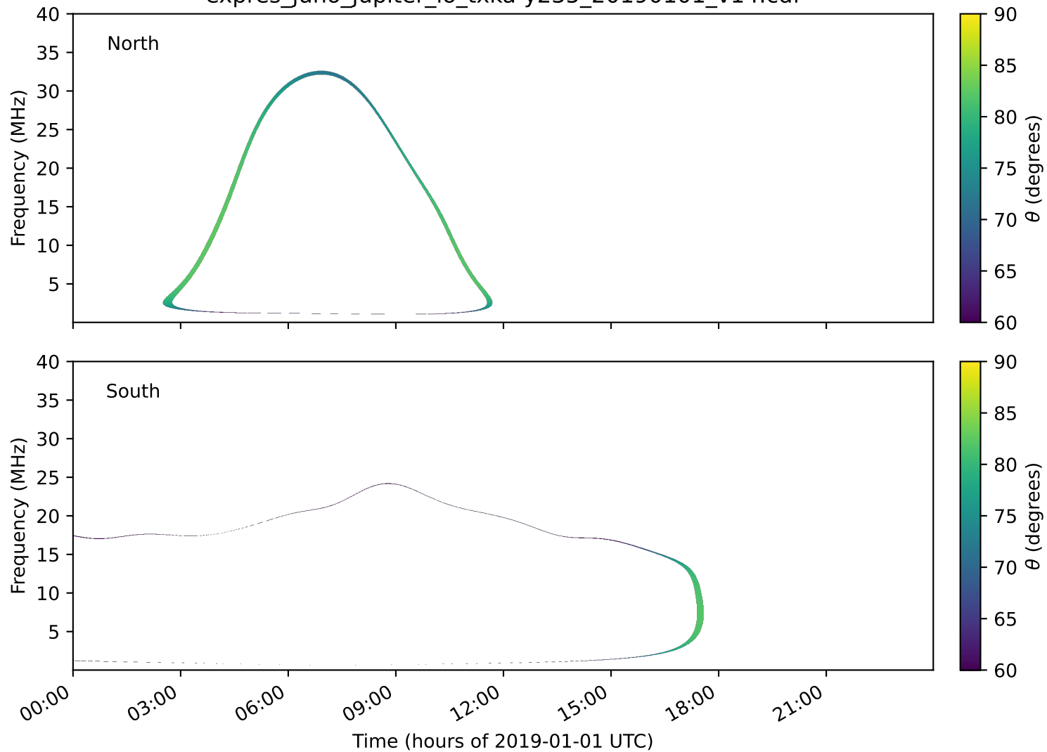
expres_juno_jupiter_io_txka-y235_20190101_v14.cdf
