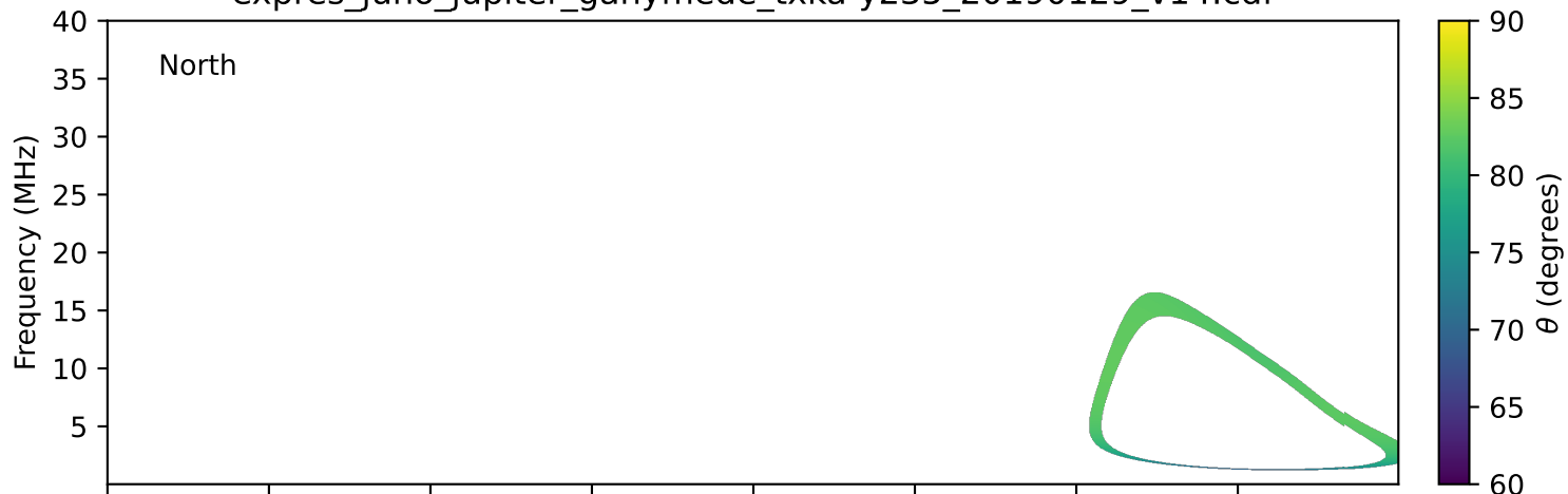
expres_juno_jupiter_ganymede_txka-y235_20190129_v14.cdf
