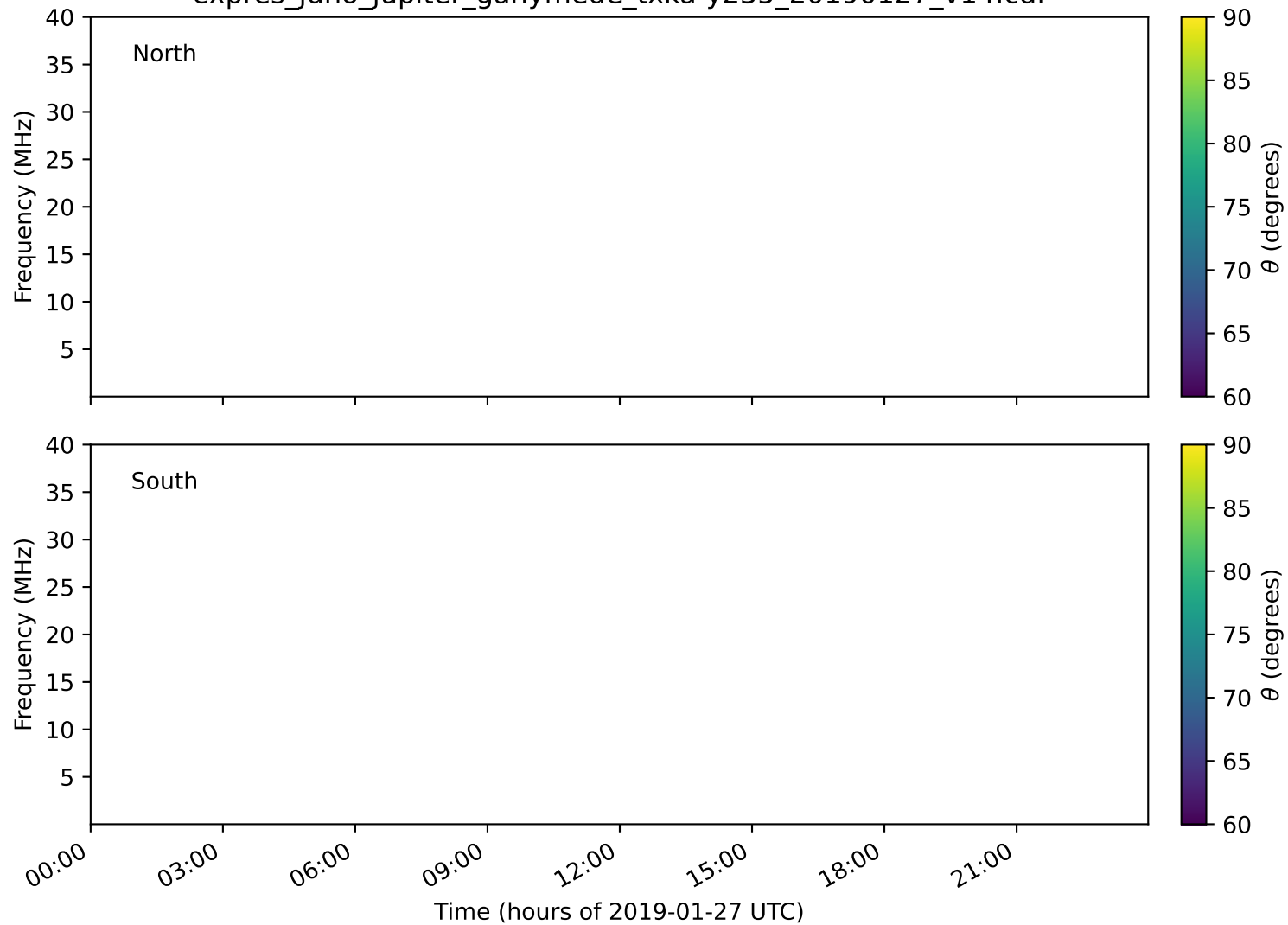
expres_juno_jupiter_ganymede_txka-y235_20190127_v14.cdf
