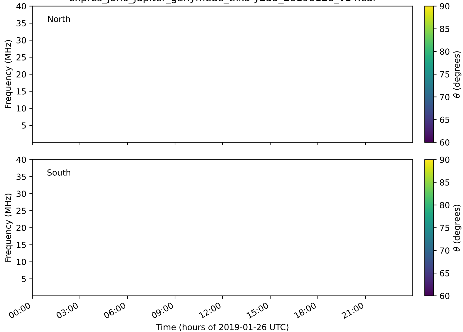
expres_juno_jupiter_ganymede_txka-y235_20190126_v14.cdf
