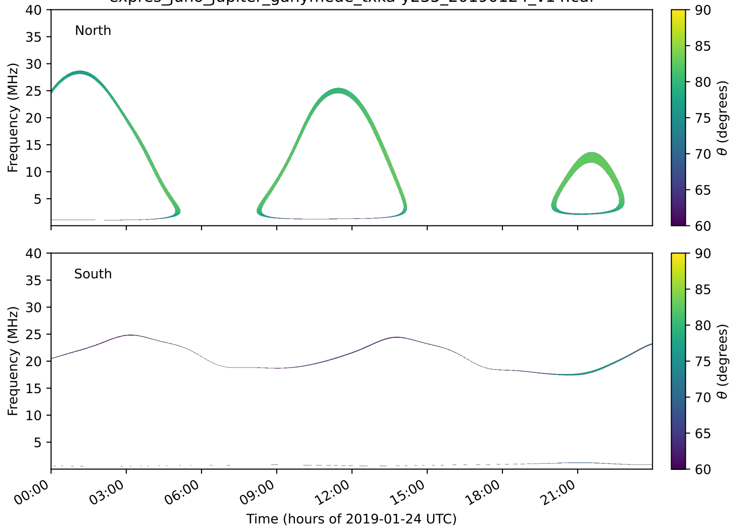
expres_juno_jupiter_ganymede_txka-y235_20190124_v14.cdf
