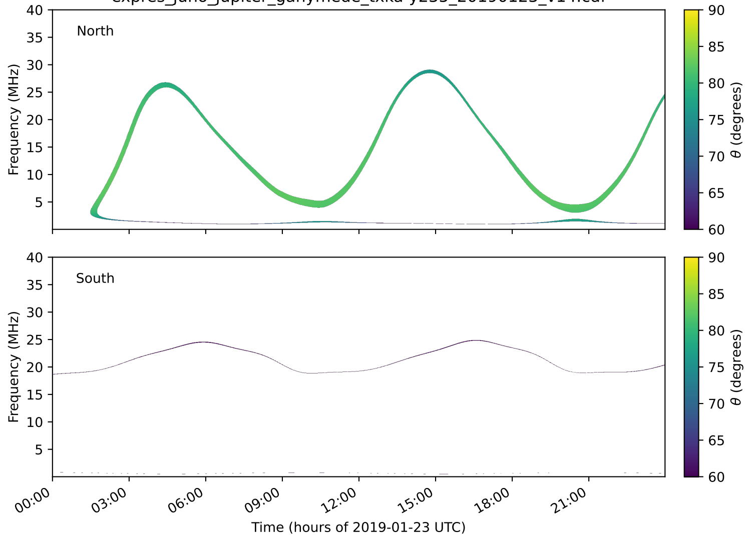
expres_juno_jupiter_ganymede_txka-y235_20190123_v14.cdf
