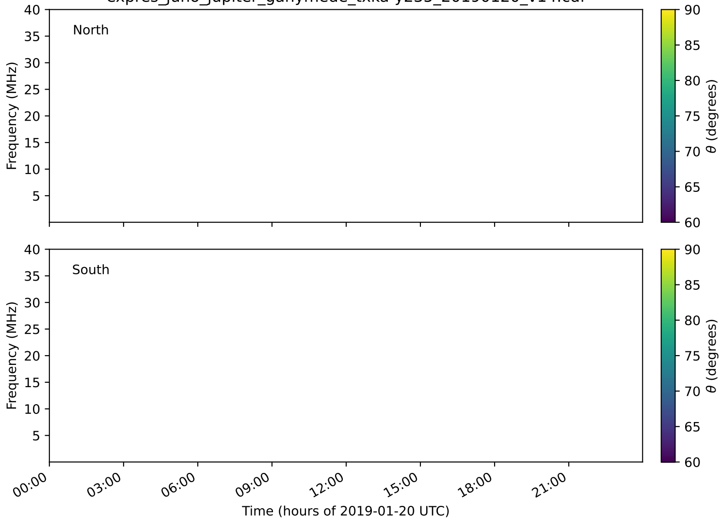
expres_juno_jupiter_ganymede_txka-y235_20190120_v14.cdf
