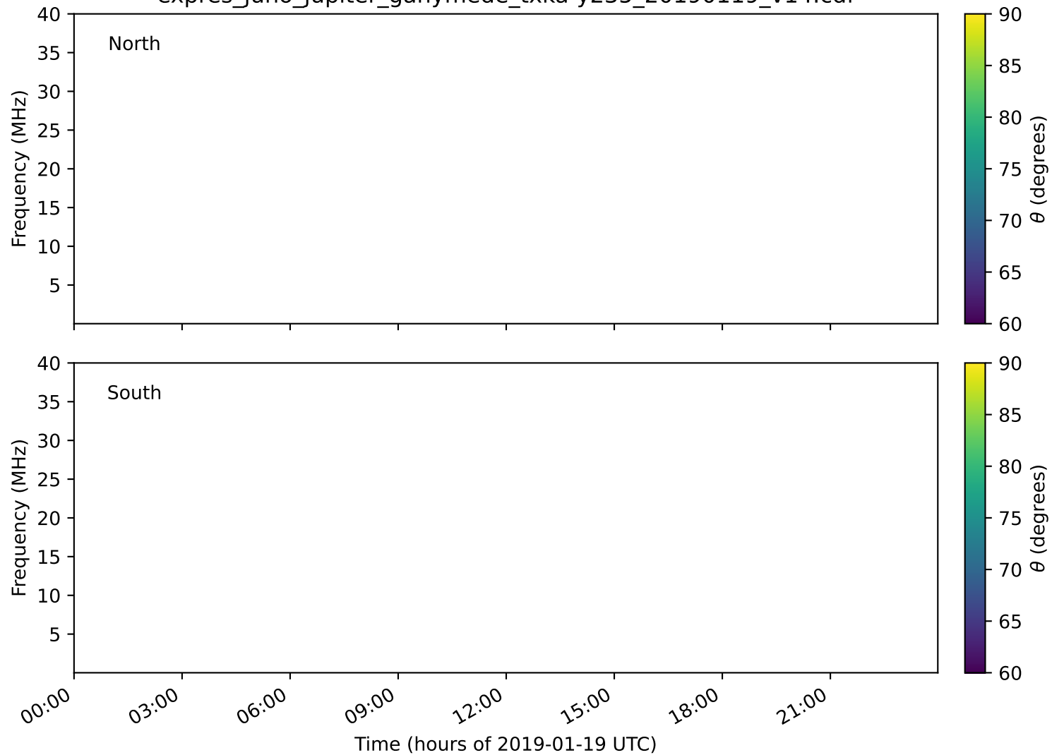
expres_juno_jupiter_ganymede_txka-y235_20190119_v14.cdf
