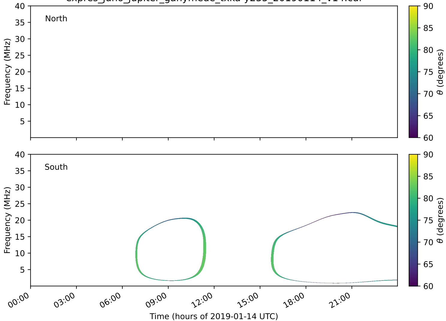
expres_juno_jupiter_ganymede_txka-y235_20190114_v14.cdf
