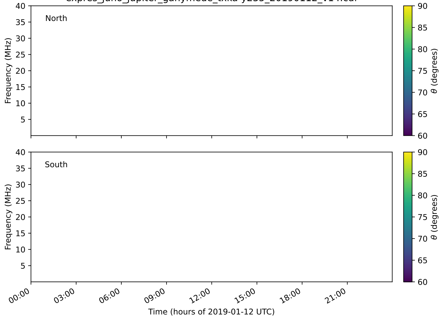
expres_juno_jupiter_ganymede_txka-y235_20190112_v14.cdf
