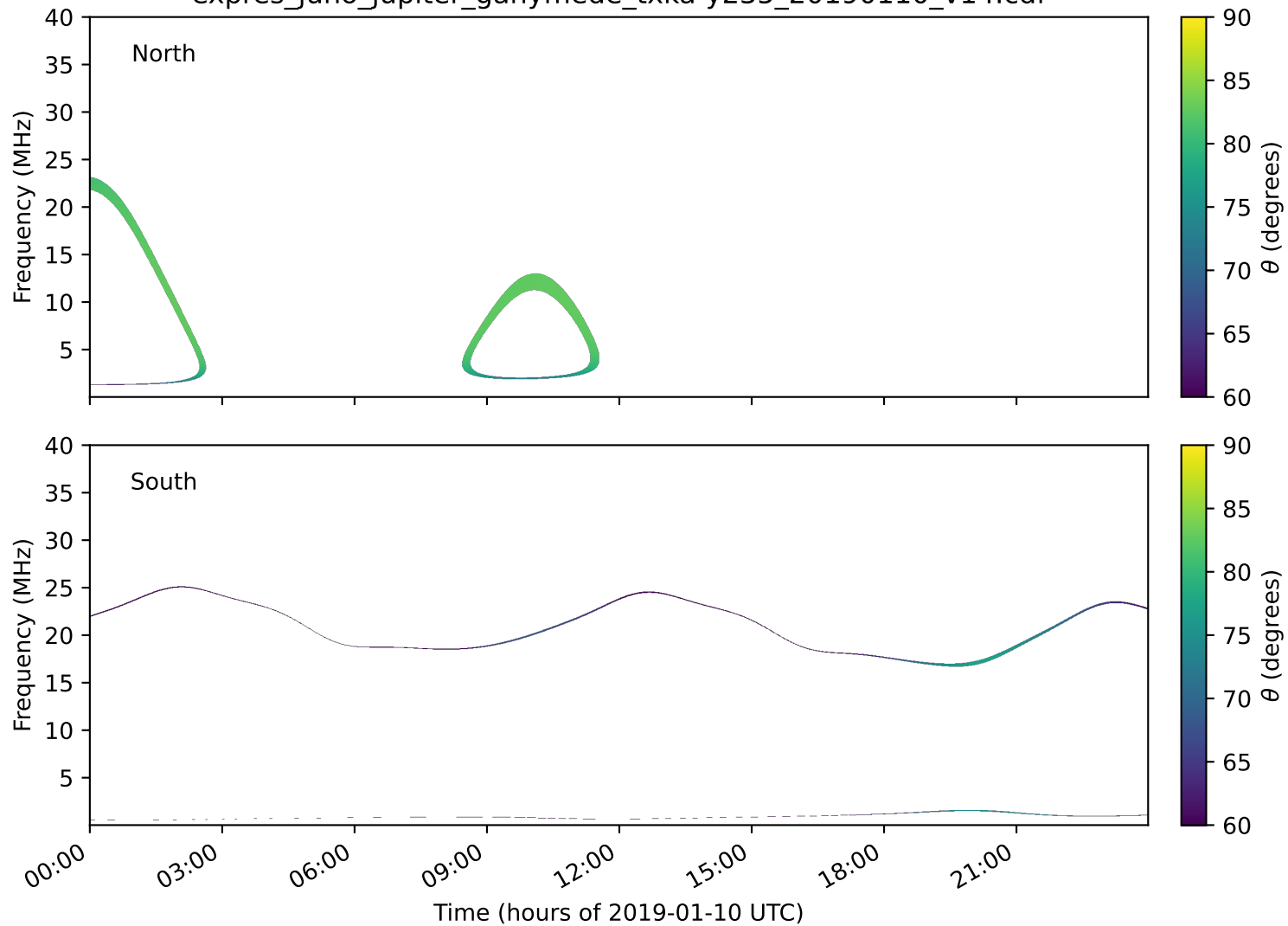
expres_juno_jupiter_ganymede_txka-y235_20190110_v14.cdf
