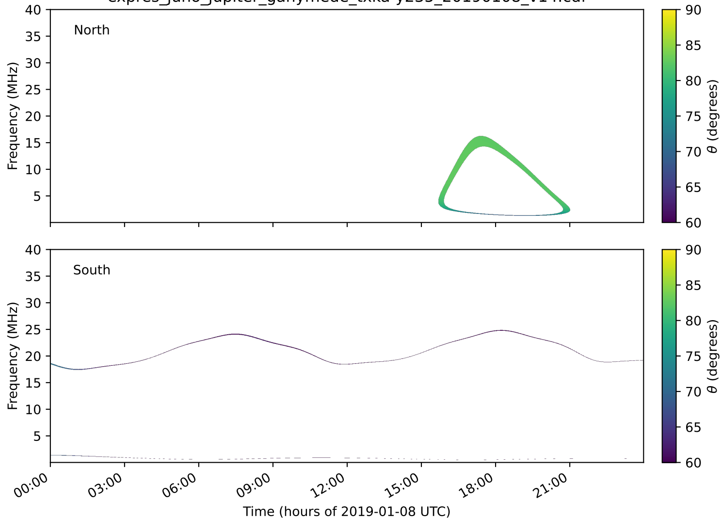
expres_juno_jupiter_ganymede_txka-y235_20190108_v14.cdf
