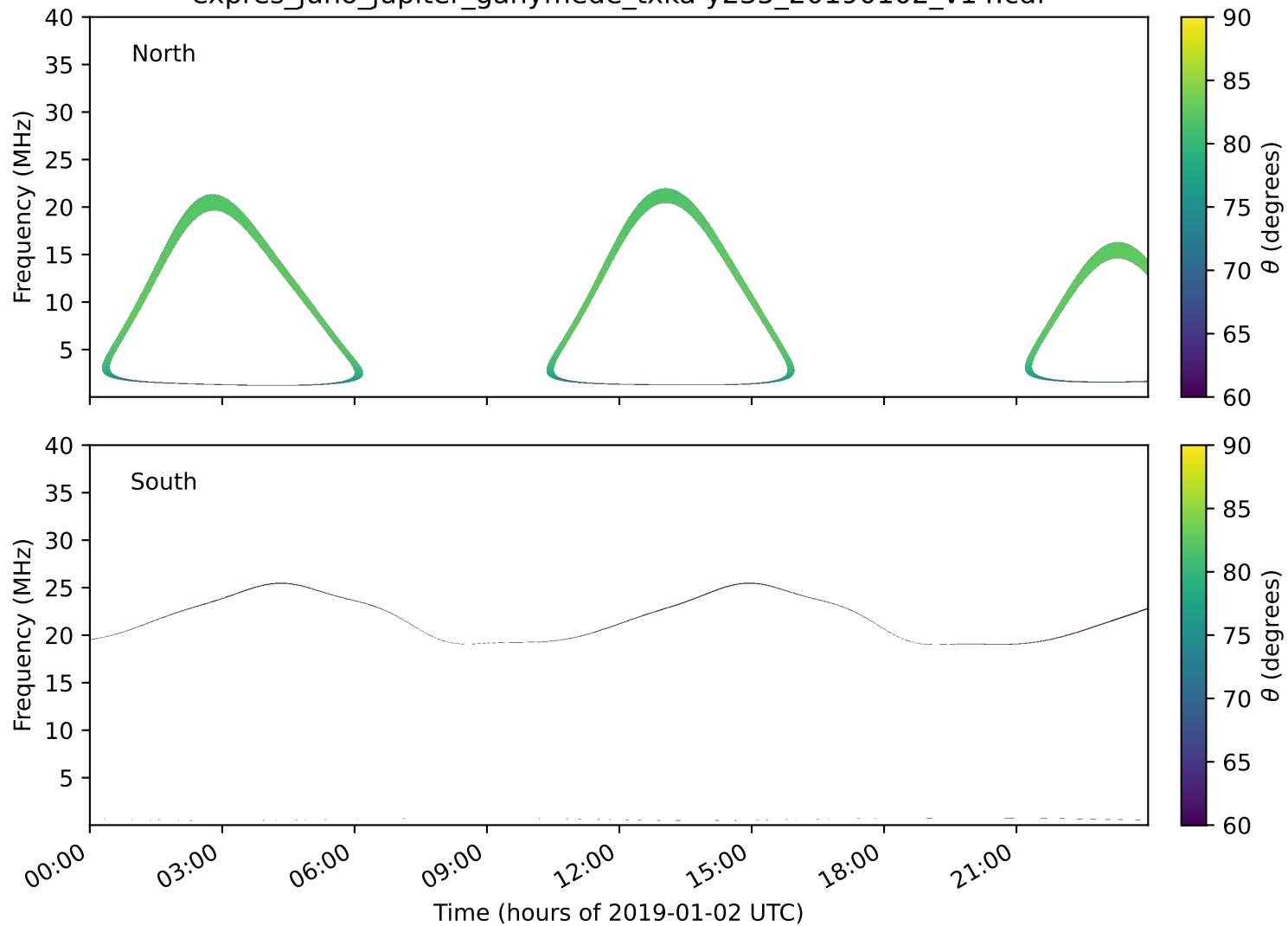
expres_juno_jupiter_ganymede_txka-y235_20190102_v14.cdf
