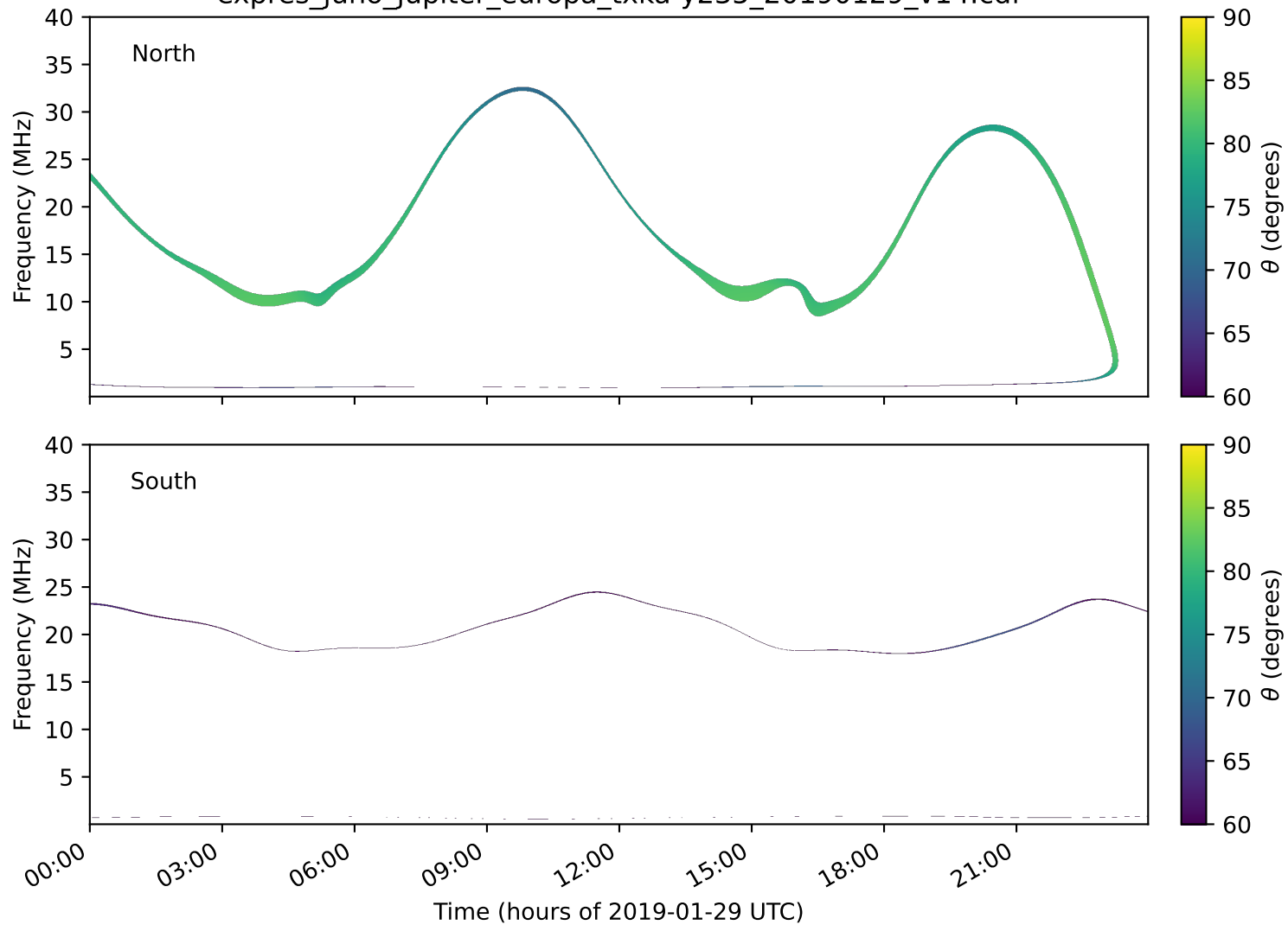
expres_juno_jupiter_europa_txka-y235_20190129_v14.cdf
