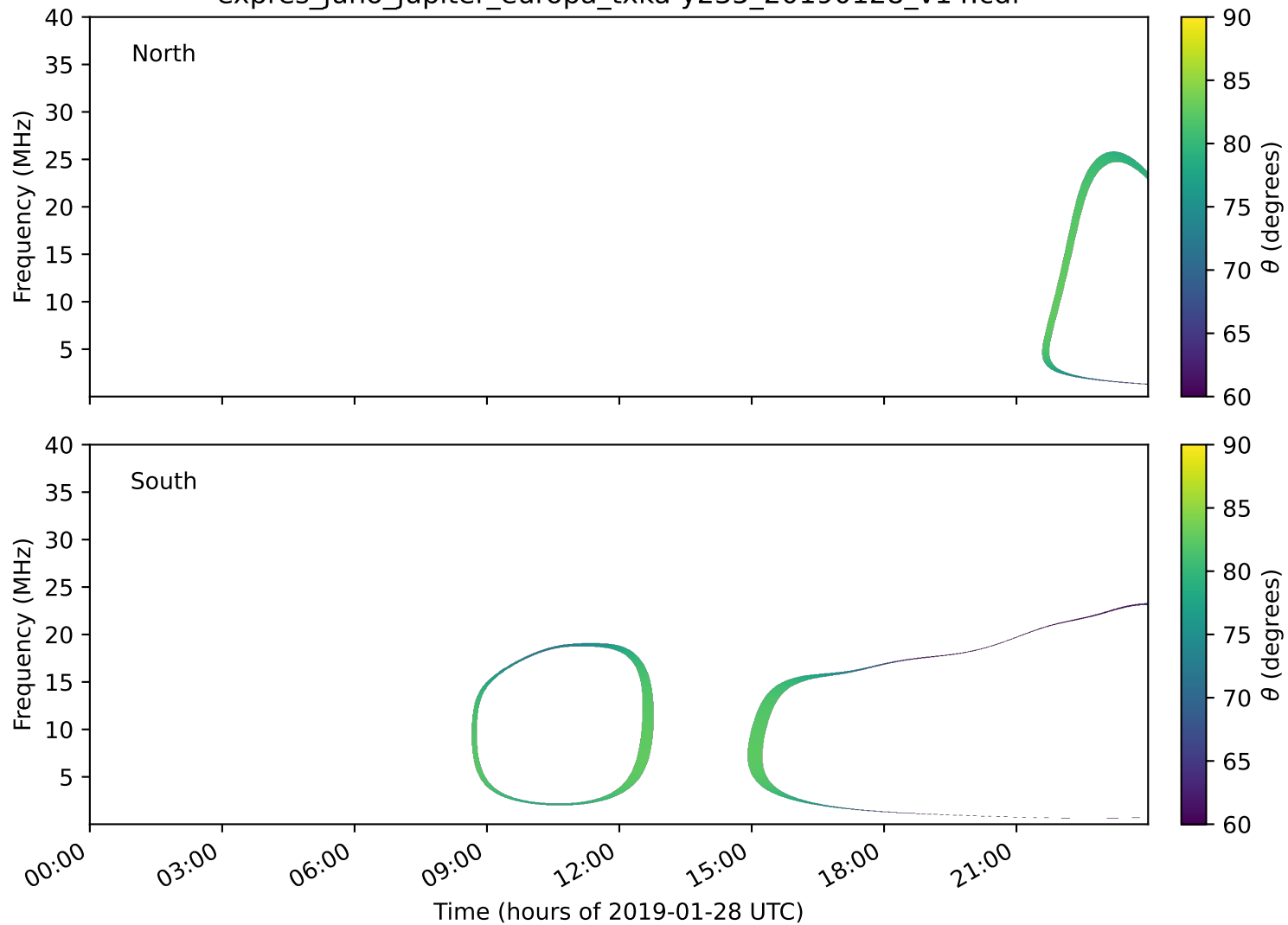
expres_juno_jupiter_europa_txka-y235_20190128_v14.cdf
