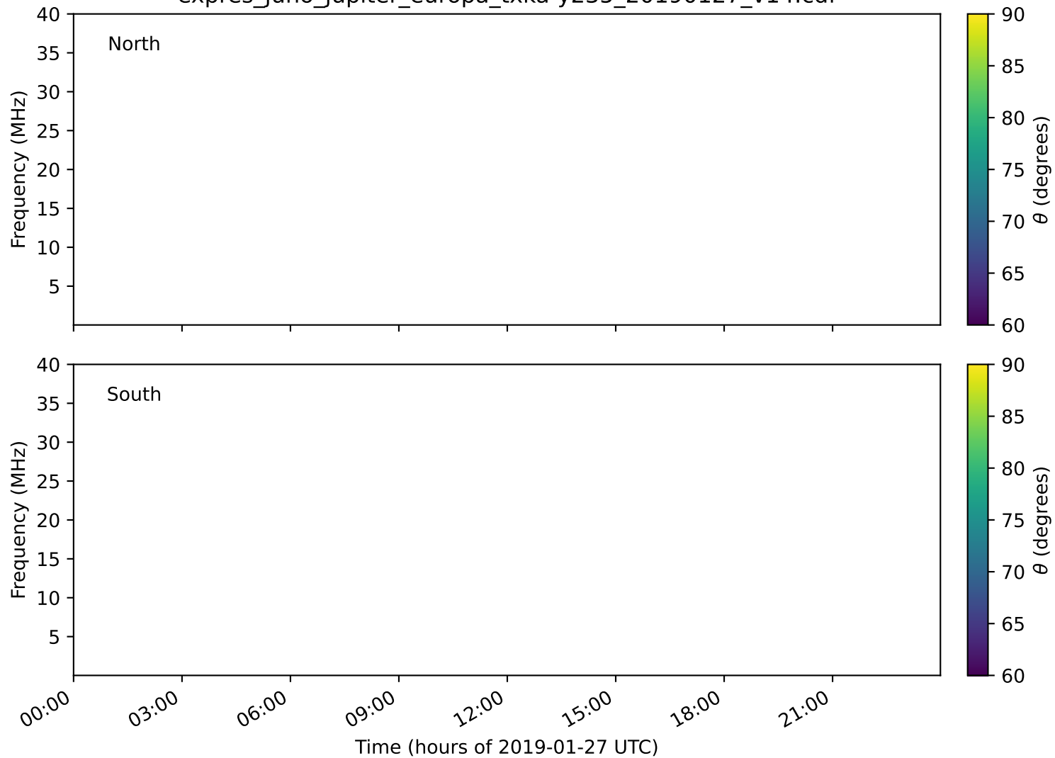
expres_juno_jupiter_europa_txka-y235_20190127_v14.cdf
