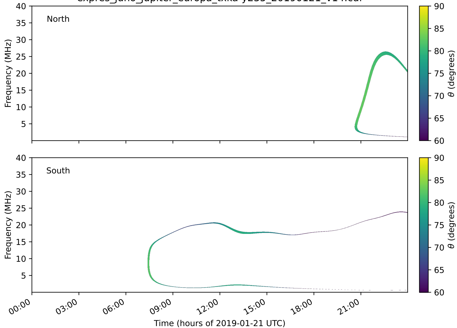
expres_juno_jupiter_europa_txka-y235_20190121_v14.cdf
