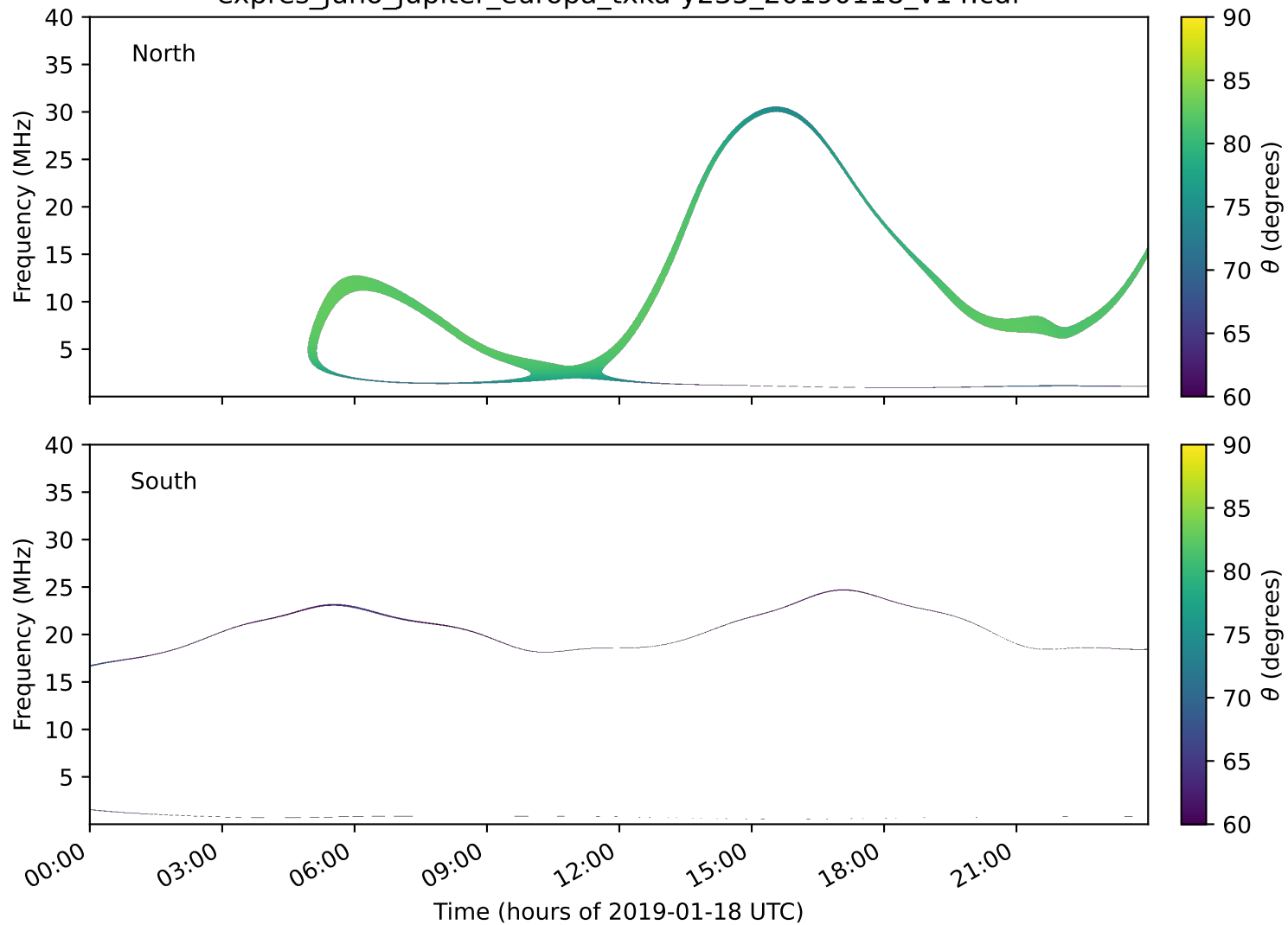
expres_juno_jupiter_europa_txka-y235_20190118_v14.cdf
