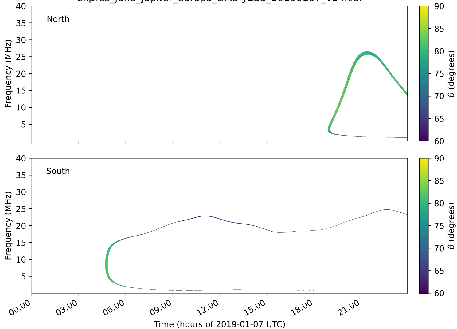
expres_juno_jupiter_europa_txka-y235_20190107_v14.cdf
