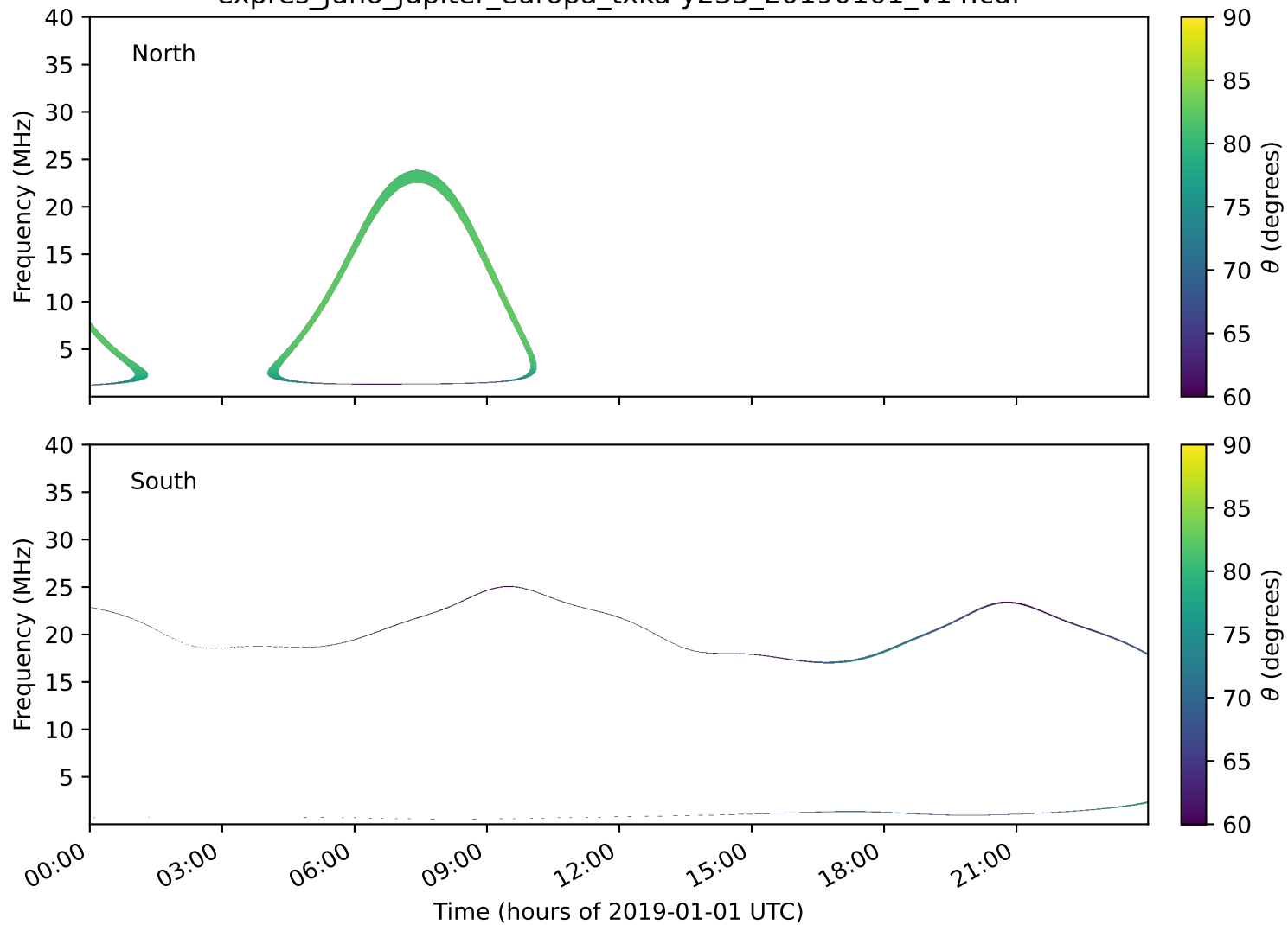
expres_juno_jupiter_europa_txka-y235_20190101_v14.cdf
