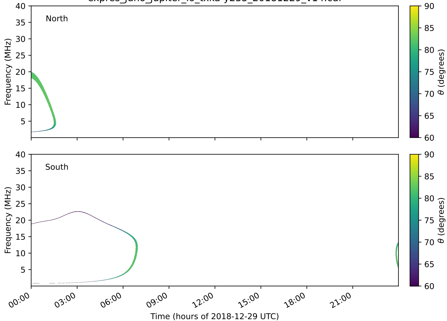
expres_juno_jupiter_io_txka-y235_20181229_v14.cdf
