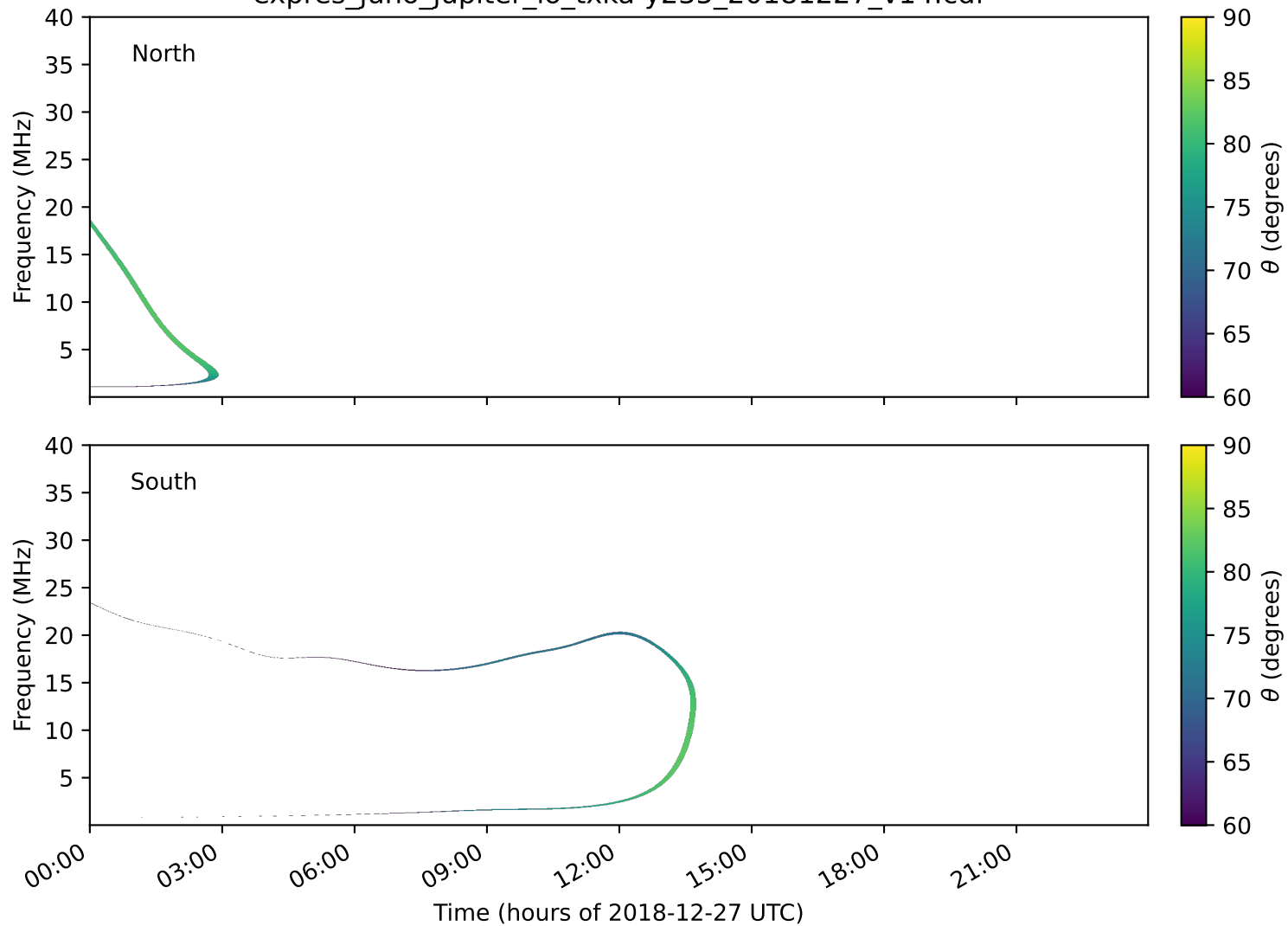
expres_juno_jupiter_io_txka-y235_20181227_v14.cdf
