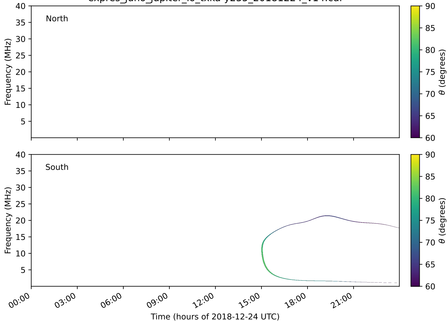
expres_juno_jupiter_io_txka-y235_20181224_v14.cdf
