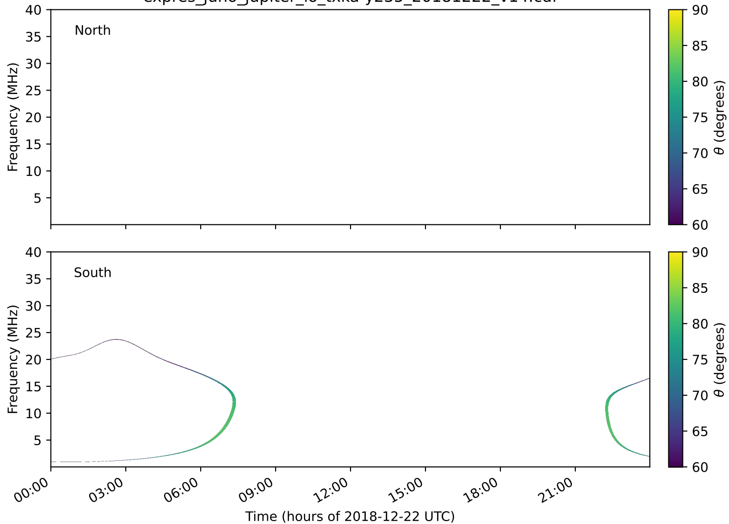
expres_juno_jupiter_io_txka-y235_20181222_v14.cdf
