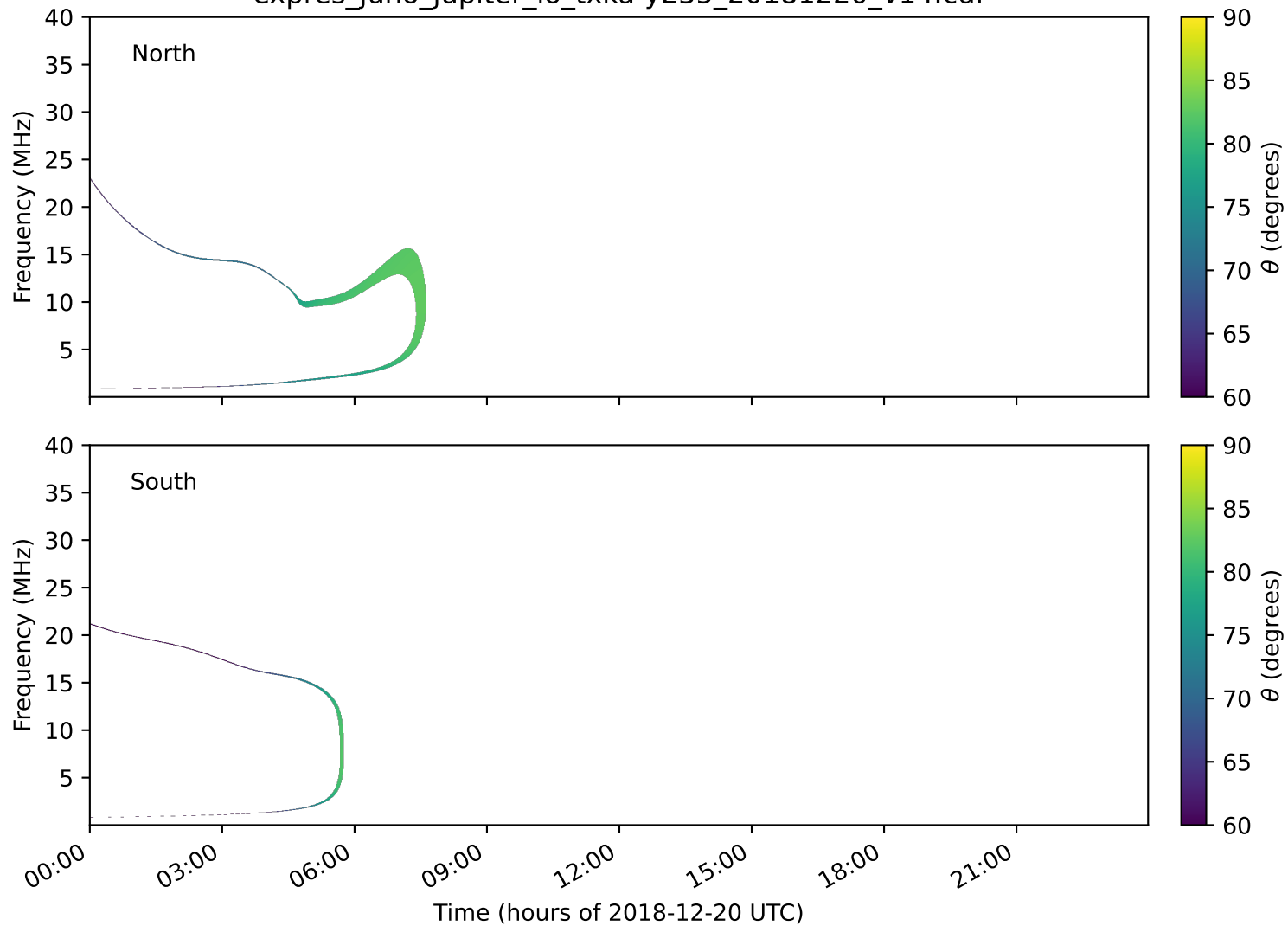
expres_juno_jupiter_io_txka-y235_20181220_v14.cdf
