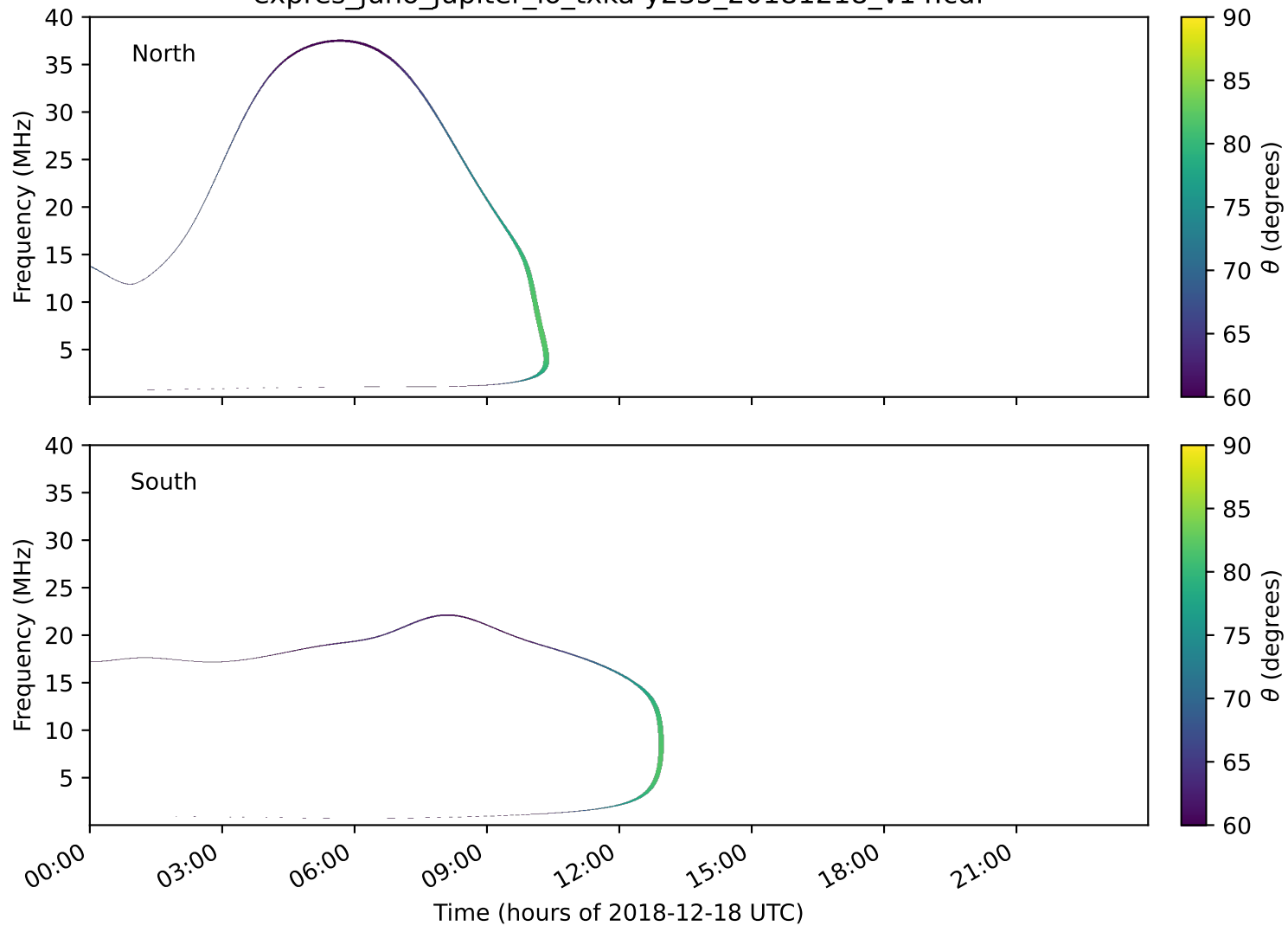
expres_juno_jupiter_io_txka-y235_20181218_v14.cdf
