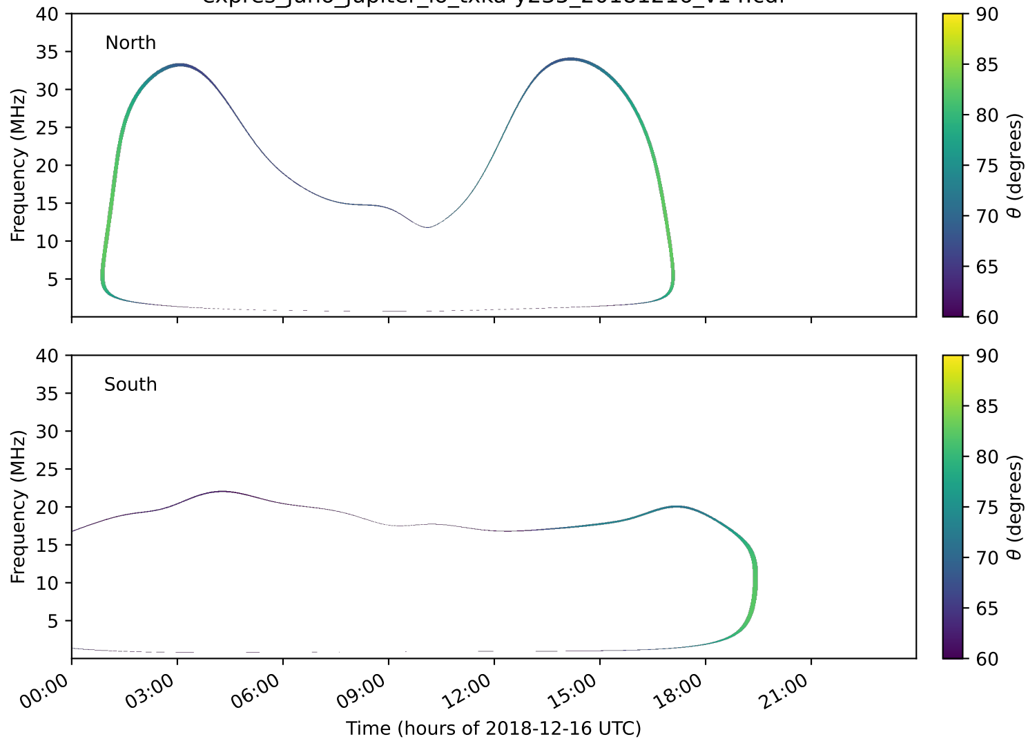
expres_juno_jupiter_io_txka-y235_20181216_v14.cdf
