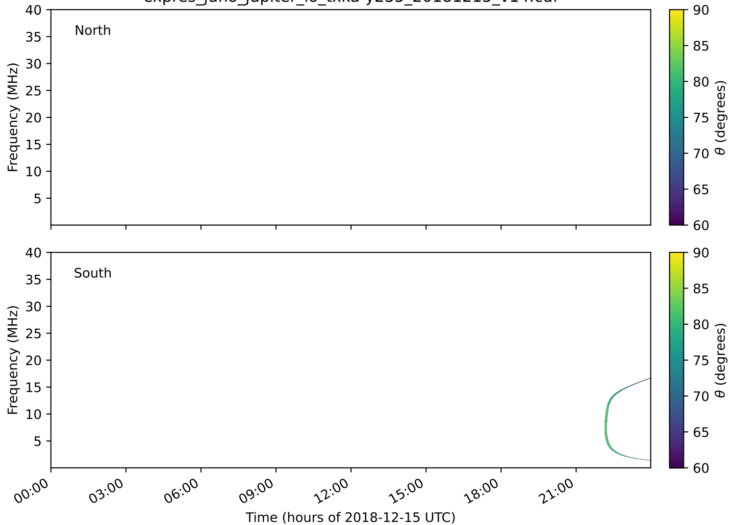
expres_juno_jupiter_io_txka-y235_20181215_v14.cdf
