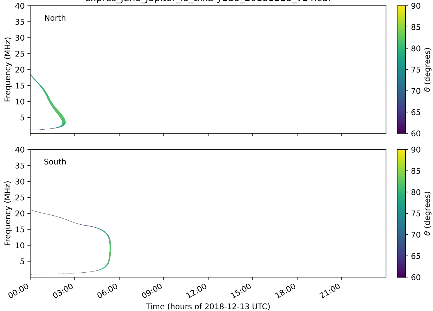
expres_juno_jupiter_io_txka-y235_20181213_v14.cdf
