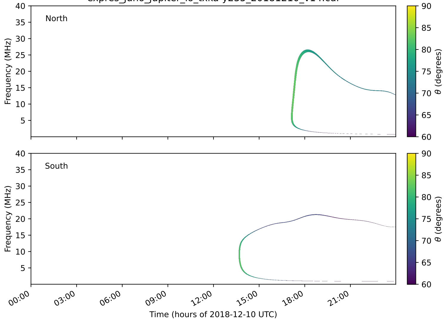
expres_juno_jupiter_io_txka-y235_20181210_v14.cdf
