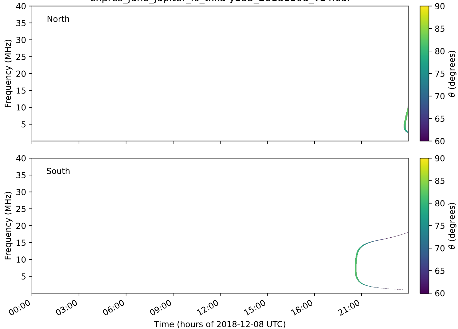
expres_juno_jupiter_io_txka-y235_20181208_v14.cdf
