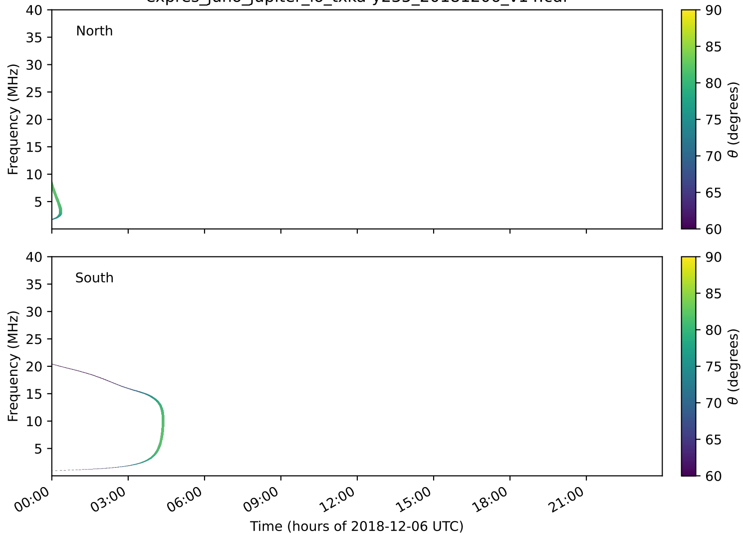
expres_juno_jupiter_io_txka-y235_20181206_v14.cdf
