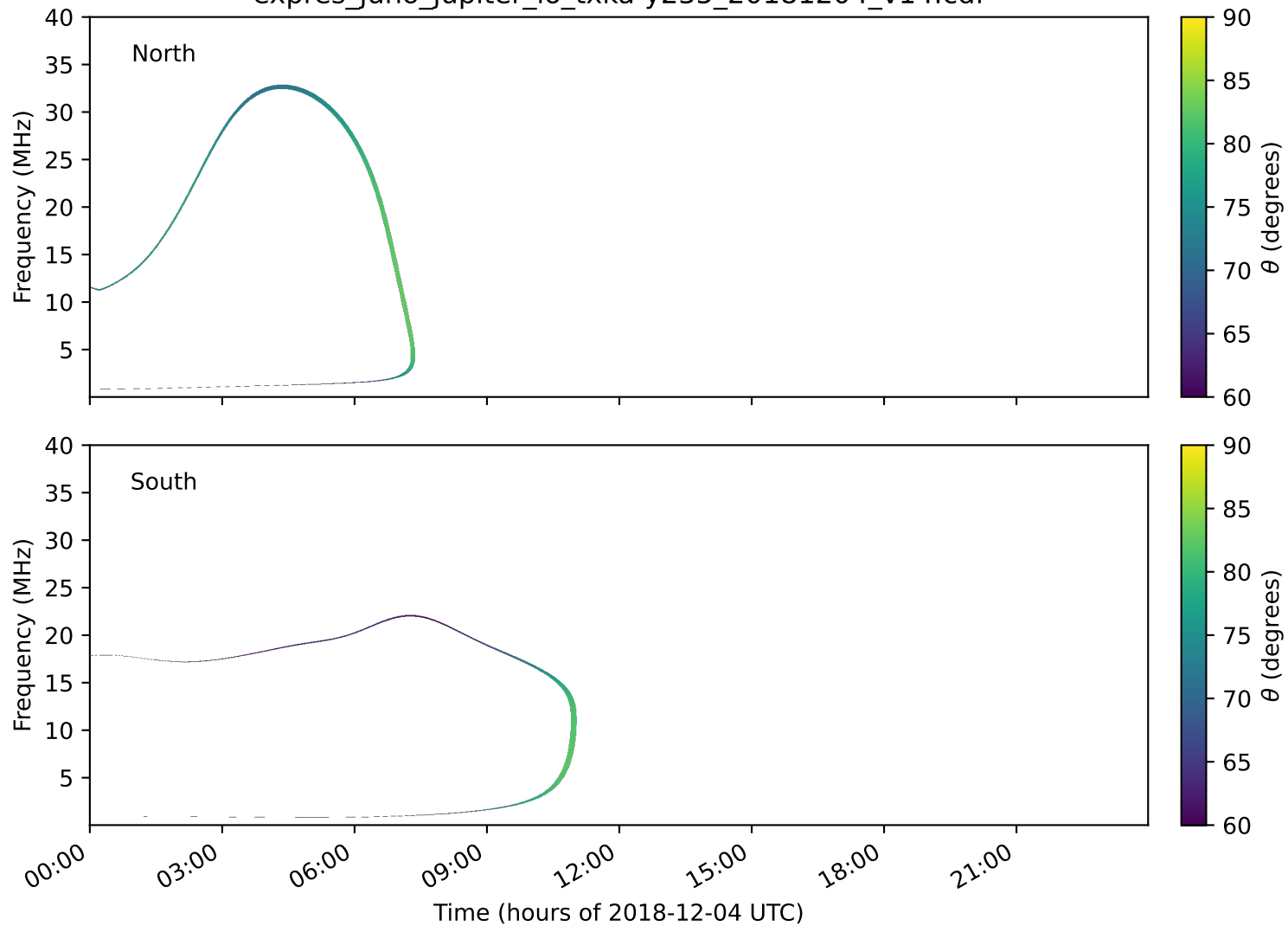
expres_juno_jupiter_io_txka-y235_20181204_v14.cdf
