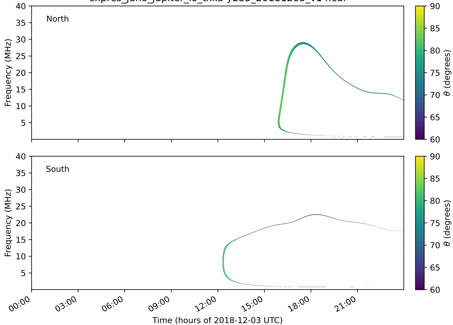
expres_juno_jupiter_io_txka-y235_20181203_v14.cdf
