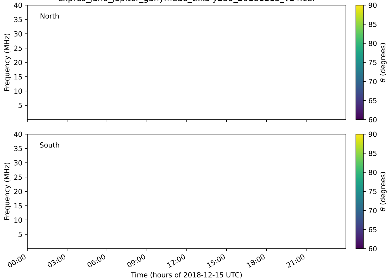
expres_juno_jupiter_ganymede_txka-y235_20181215_v14.cdf
