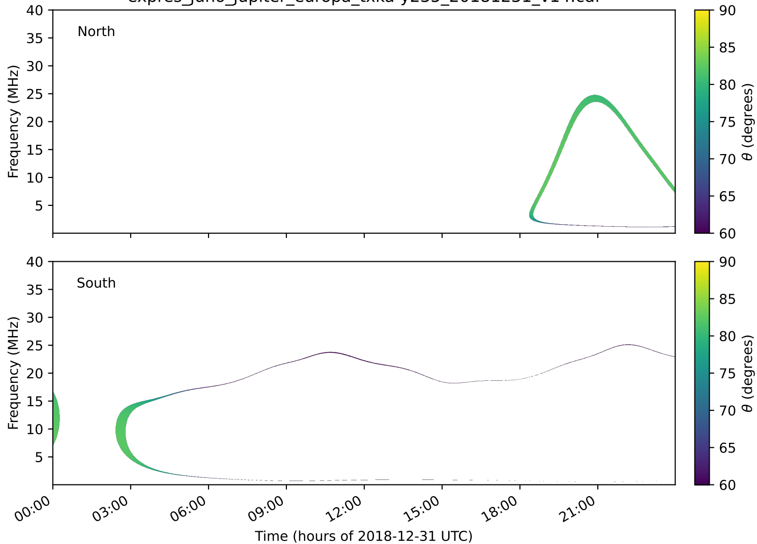
expres_juno_jupiter_europa_txka-y235_20181231_v14.cdf
