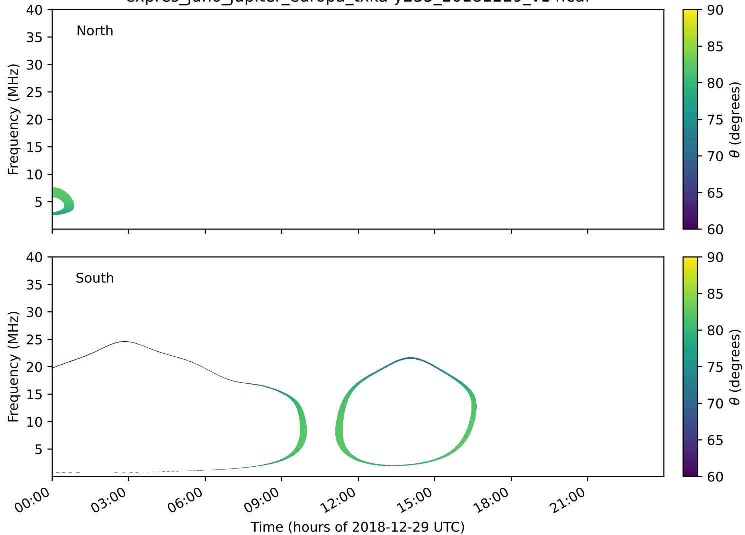
expres_juno_jupiter_europa_txka-y235_20181229_v14.cdf
