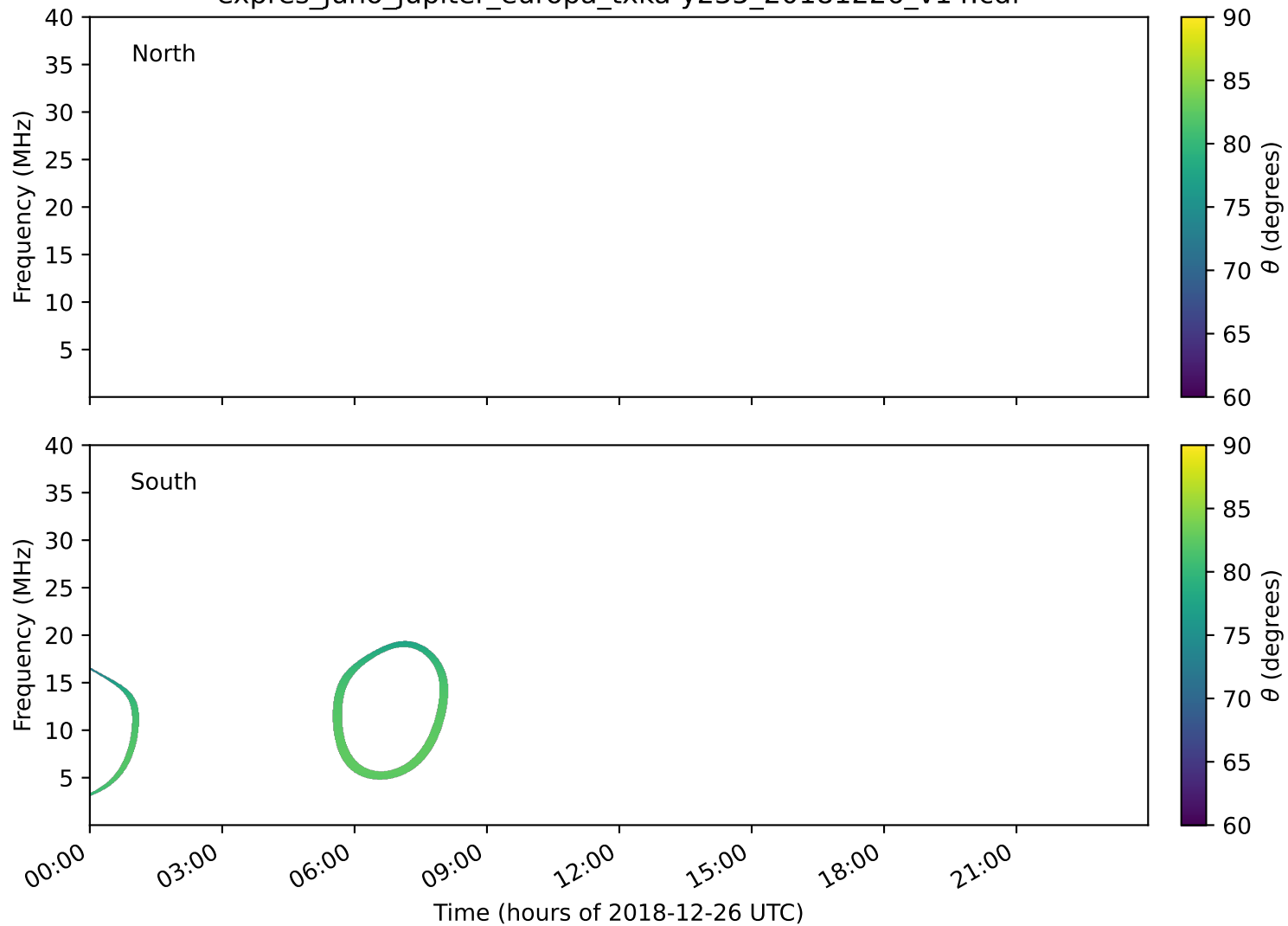
expres_juno_jupiter_europa_txka-y235_20181226_v14.cdf
