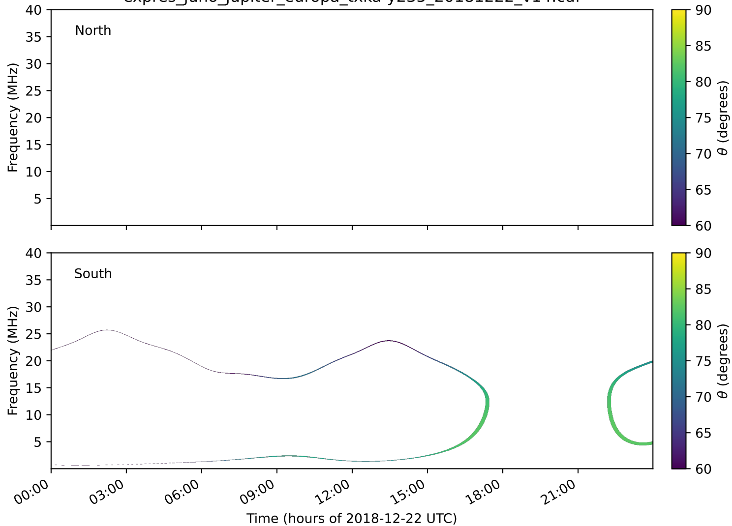
expres_juno_jupiter_europa_txka-y235_20181222_v14.cdf
