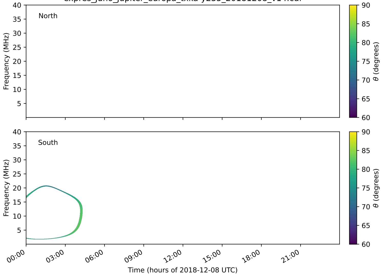
expres_juno_jupiter_europa_txka-y235_20181208_v14.cdf
